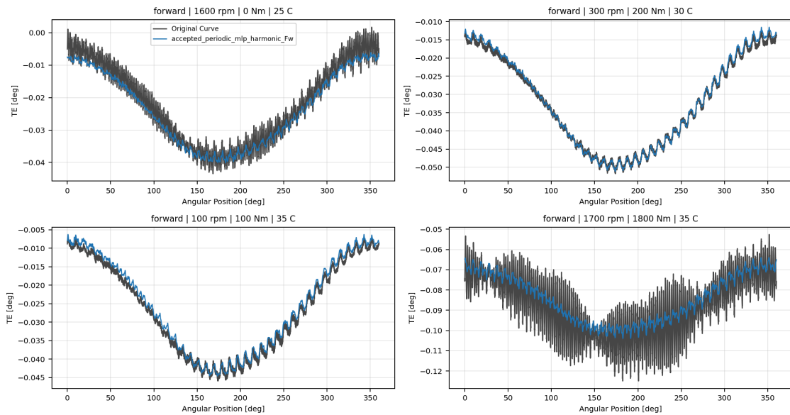
Forward Accepted Non Windowed Reference Overlay TE Curve Verification Pipeline comparison
