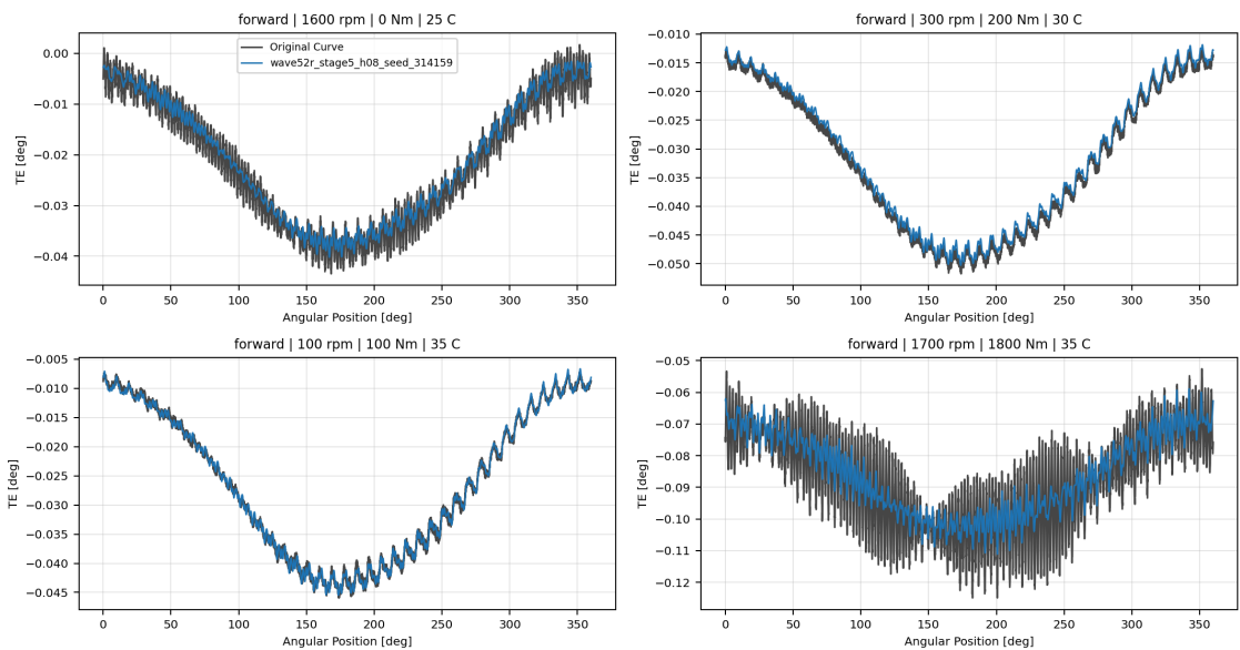
Forward Wave52r Stage5 Non Temporal Overlay TE Curve Verification Pipeline comparison
