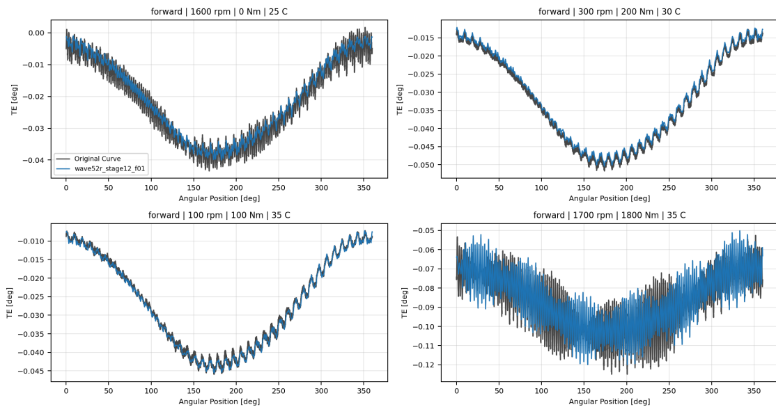
Forward Wave52r Stage12 Temporal Overlay TE Curve Verification Pipeline comparison
