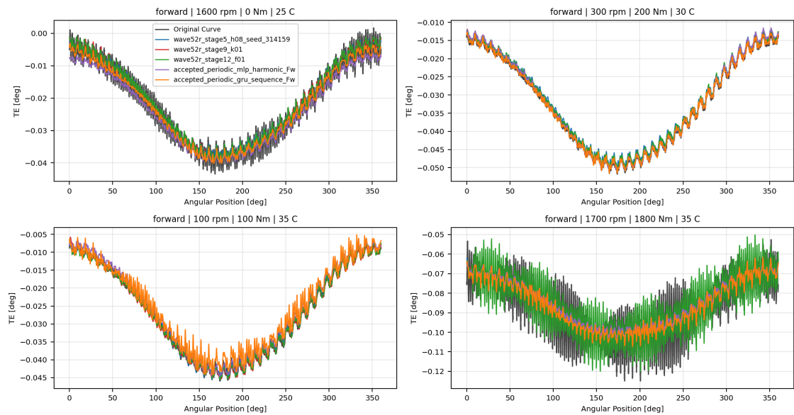
Forward Wave 5.2R Cross-Lane Finalist Overlay TE Curve Verification Pipeline comparison
