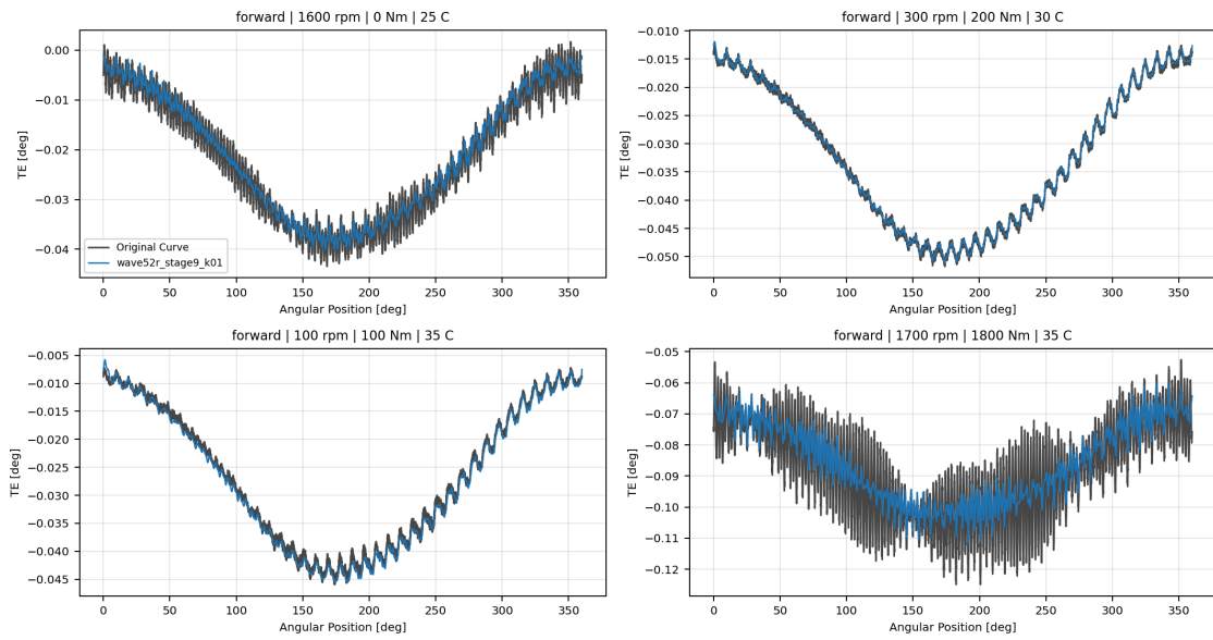
Forward Wave52r Stage9 Temporal Overlay TE Curve Verification Pipeline comparison
