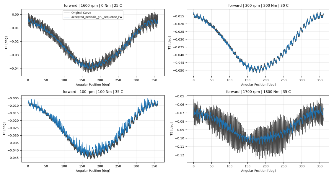
Forward Accepted Time Windowed Incumbent Overlay TE Curve Verification Pipeline comparison
